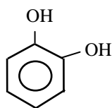
pirocatecol
